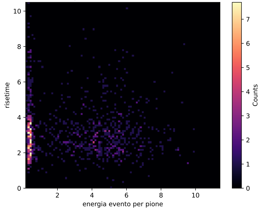
pion distribution 10.0GeV
