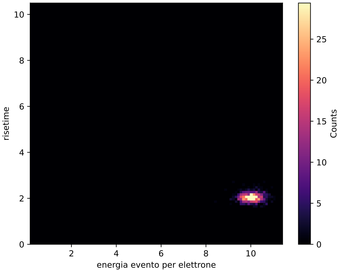
electron distribution 10.0GeV
